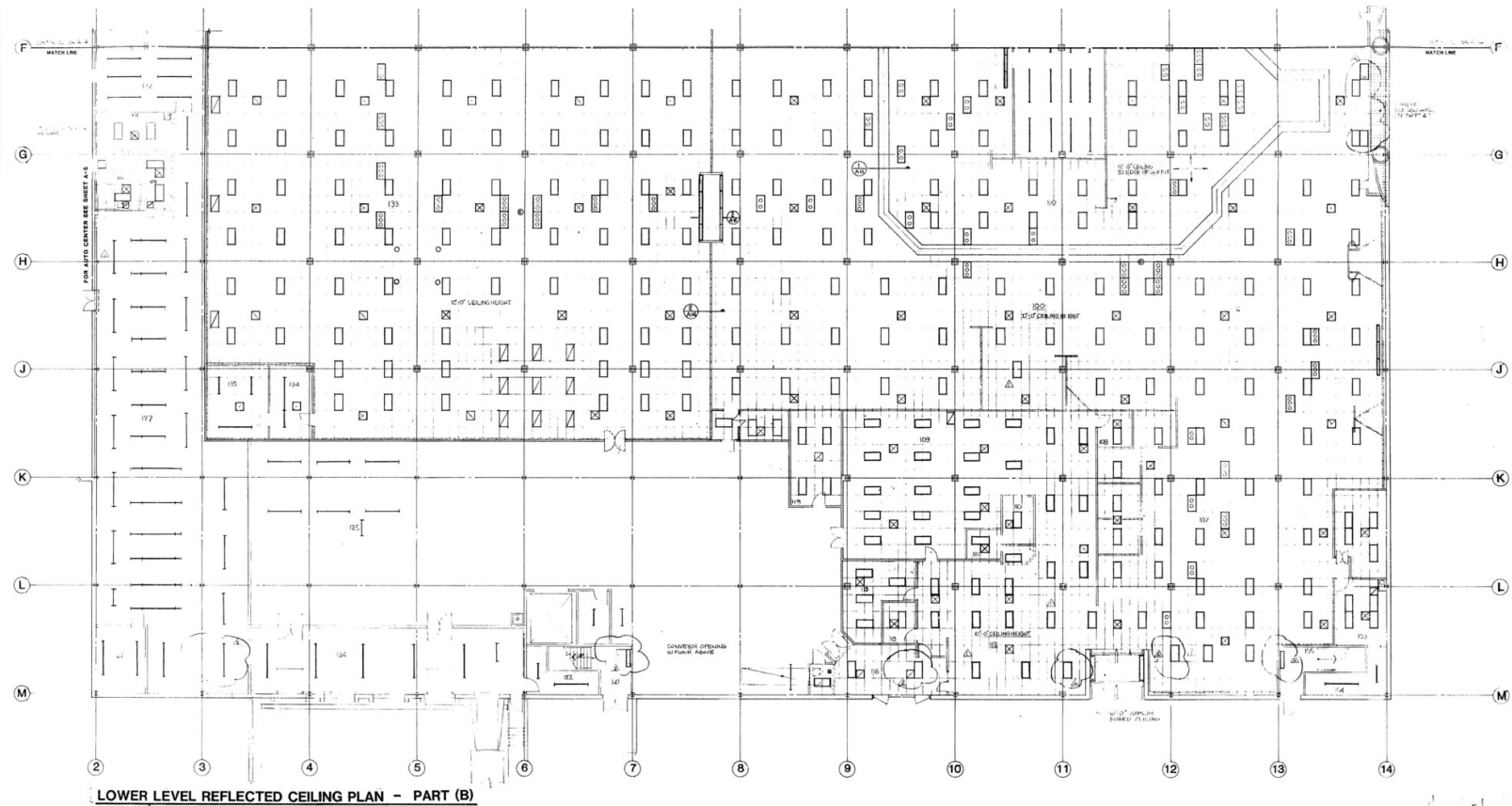
LOWER LEVEL REFLECTED CEILING PLAN - PART (B)
